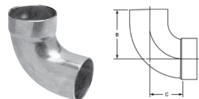
807-2 DWV 90° Fitting Elbow Ftg x C – Cast
