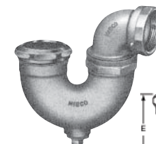
892-A DWV P-Trap w/Union Joint F x SJ x Cleanout w/Plug – Cast
