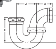
892-3 DWV P-Trap w/Union Joint F x SJ – Cast
