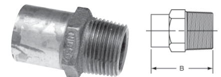
704-2 Fitting Adapter Ftg x M – Cast
