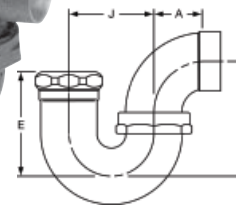
892 DWV P-Trap w/Union Joint C x SJ – Cast
