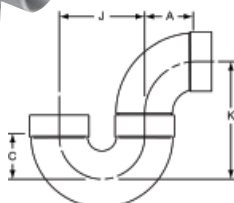
892-A DWV P-Trap w/Union Joint F x SJ x Cleanout w/Plug – Cast
