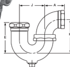
892-A DWV P-Trap w/Union Joint F x SJ x Cleanout w/Plug – Cast
