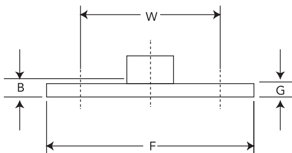
FLANGES - CLASS 150
