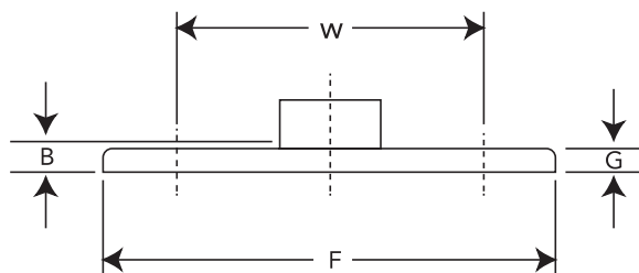
FLANGES - CLASS 125
