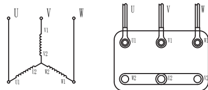
Schematic Diagram
